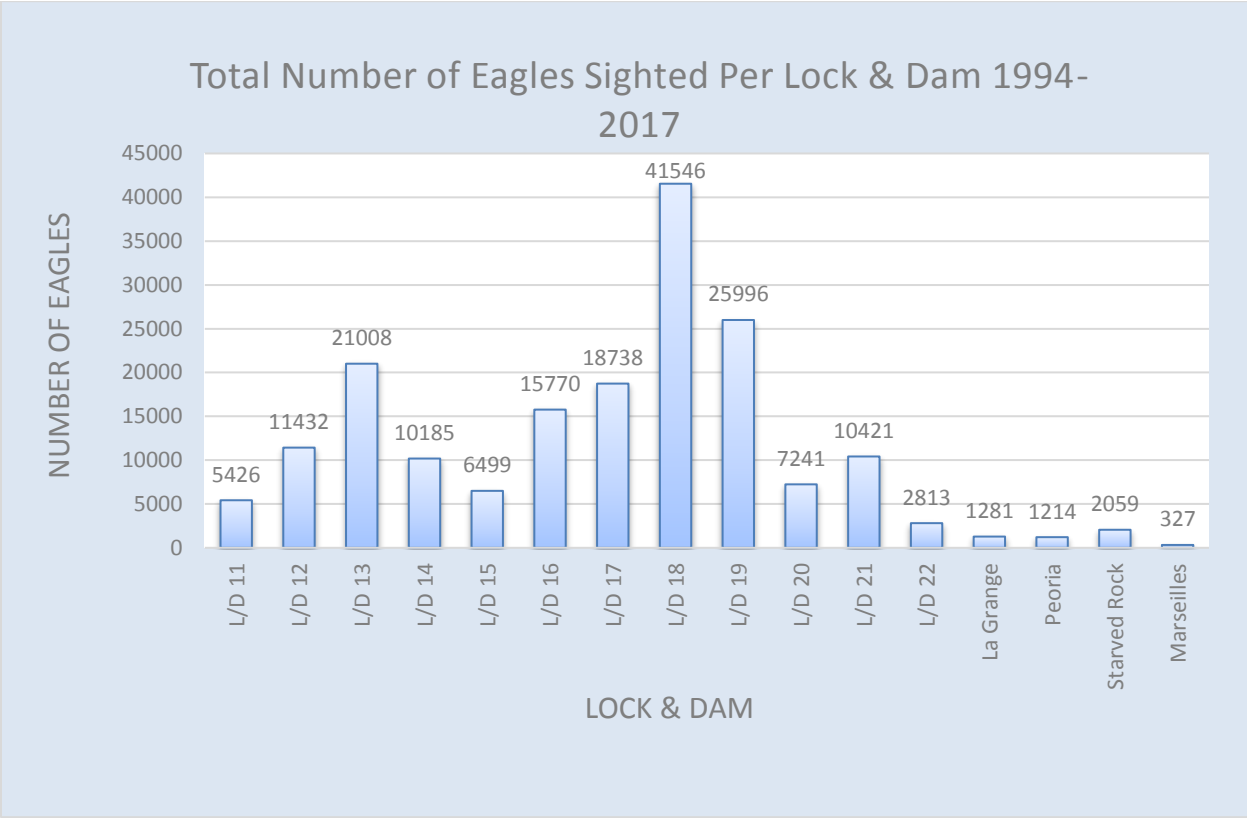
Figure 6. Eagles sighted per Lock & Dam 1994-2017 seasons
