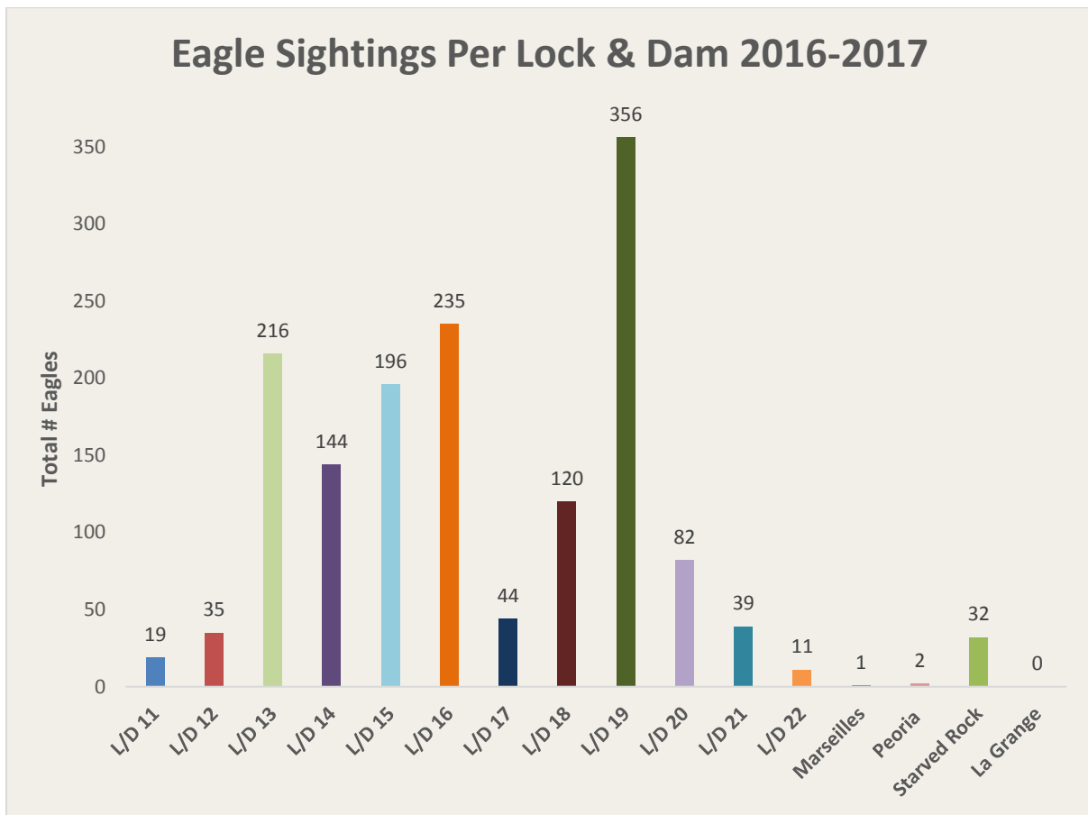
Figure 4. Bar graph showing distribution of total eagle sightings at all locks & dams during 2016-17 season
