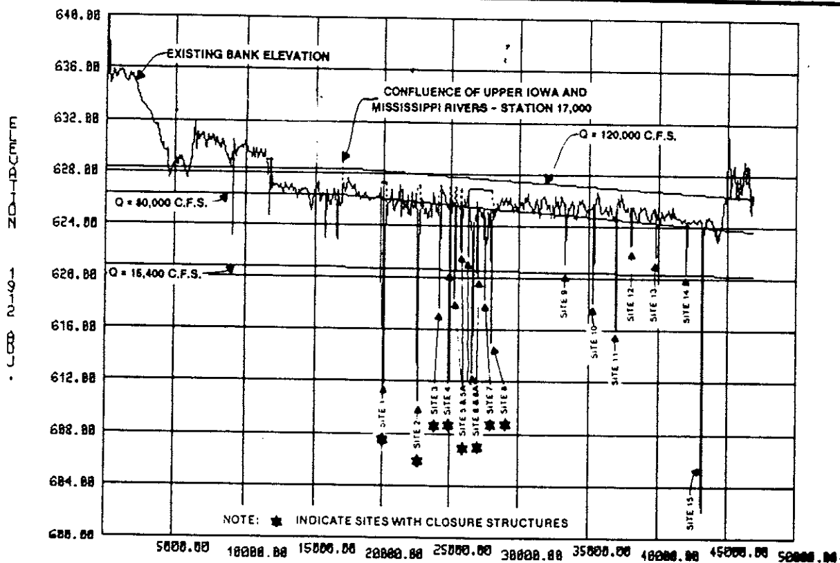
MISSISSIPPI AND UPPER IOWA RIVERS EXISTING AND PROPOSED RIGHT BANK PROFILES AND WATER SURFACE PROFILES, PLAN 1
