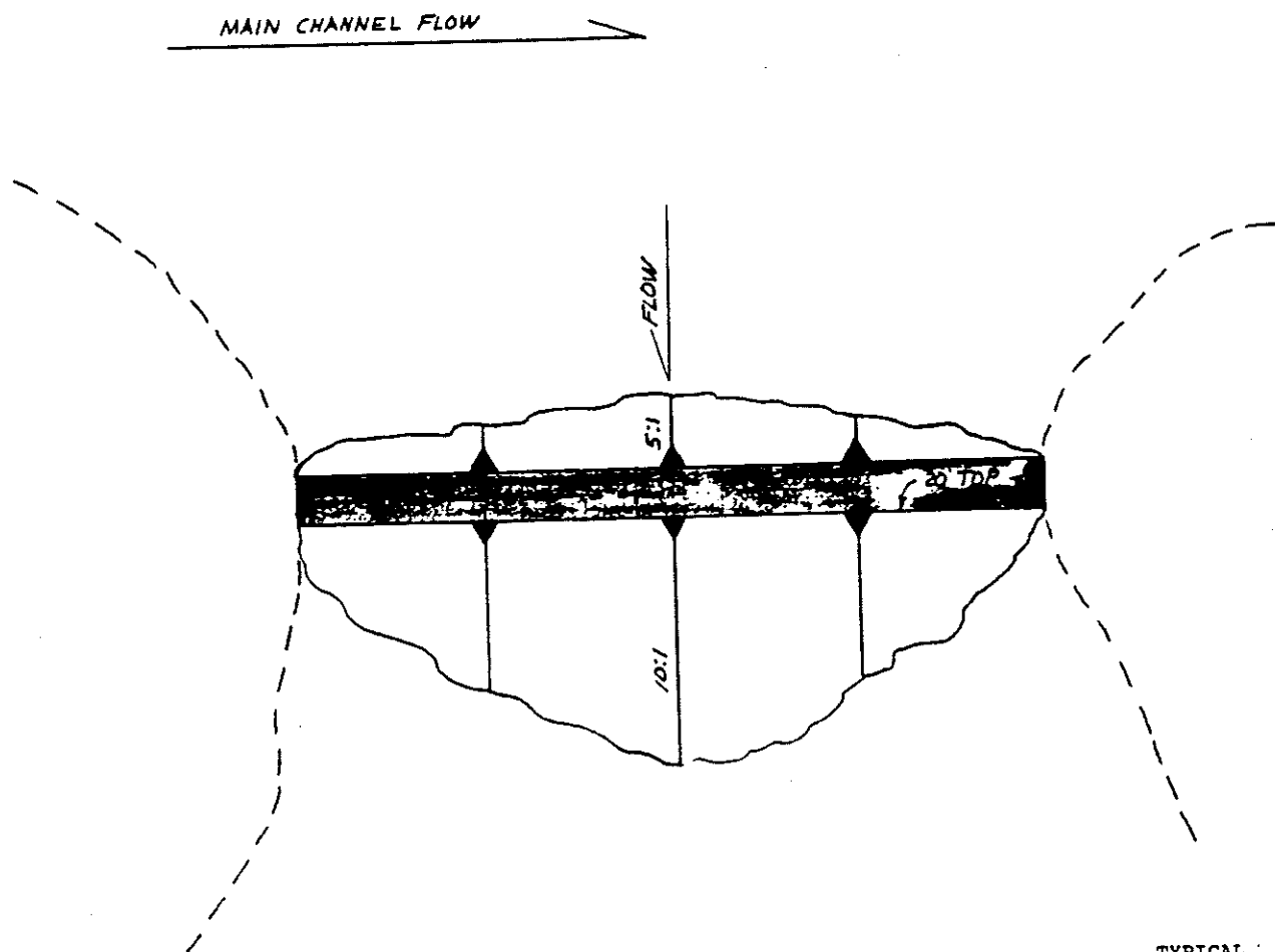
TYPICAL CHANNEL CLOSURE STRUCTURE PLAN NTS
