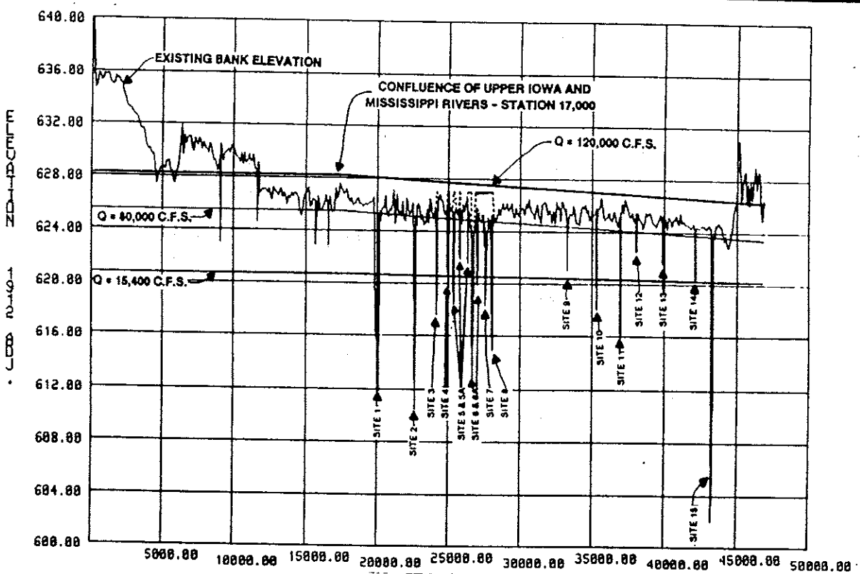
MISSISSIPPI AND UPPER IOWA RIVERS EXISTING AND PROPOSED RIGHT BANK PROFILES AND WATER SURFACE PROFILES, PLAN 5
