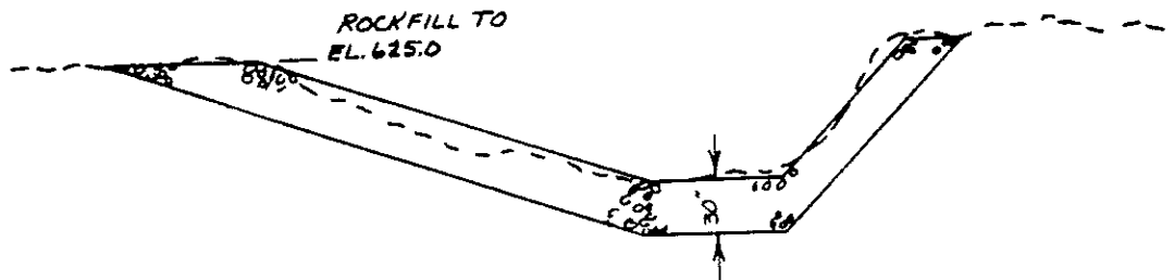
TYPICAL ROCK LINED SIDE CHANNEL SECTION NTS
