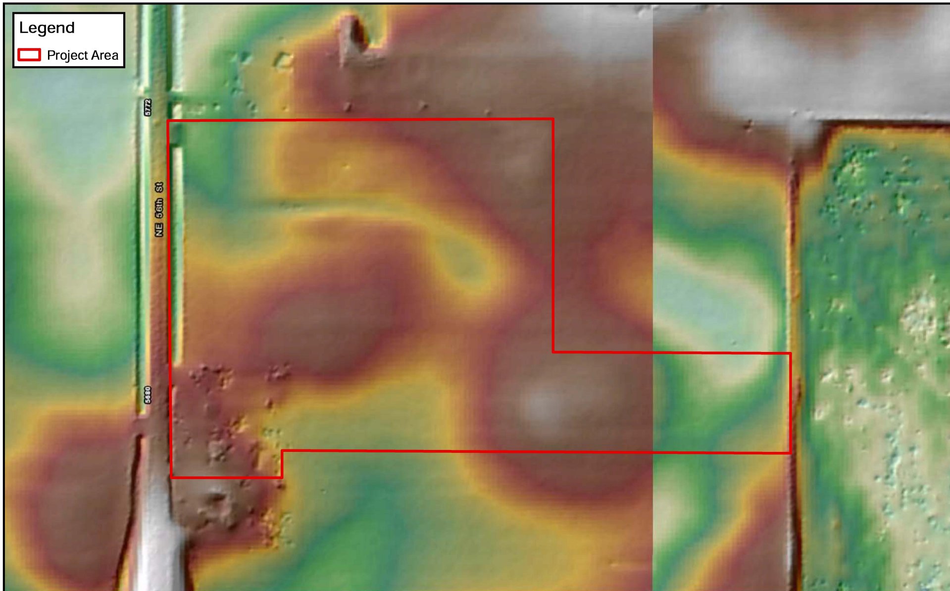
Figure 4: Hillshade Map
