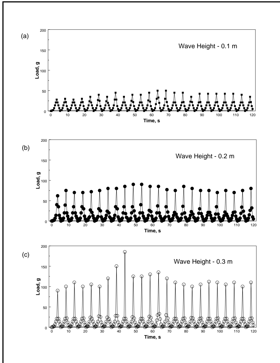
Figure 15. Tensile loading measured on an 8-week-old Eurasian watermilfoil shoot during exposure to a repeating series ( W_p = 3 sec) of waves with heights of (a) 0.1 m, (b) 0.2 m, and (c) 0.3m. (Ambient current velocity = 0.10 m/sec). Tensile load measured at base of the sheet)
