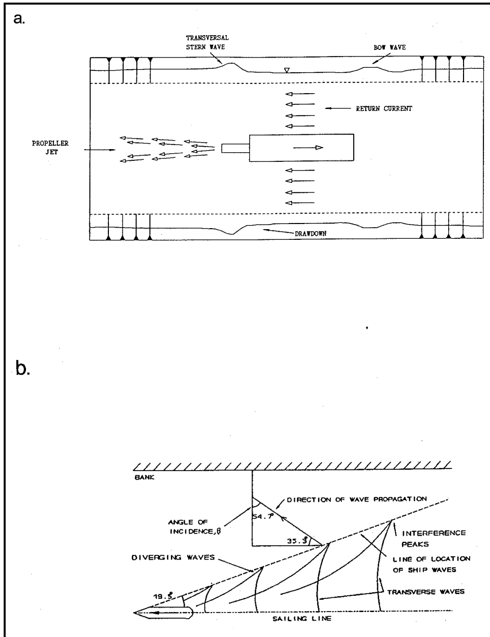
Figure 1. Type of waves and currents generated by commercial navigation traffic: (a) general definition sketch of navigation effects terms, (b) ship wave angles and definition sketch
