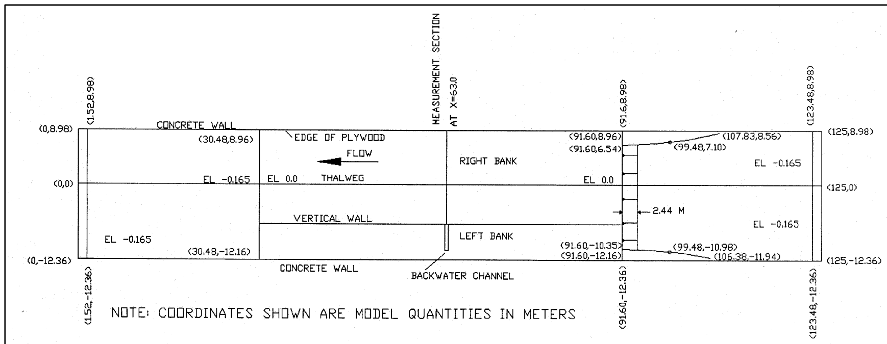
Figure 2. Flume dimensions and location of backwater
