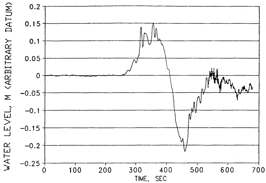
a. Wave gage located outside the backwater channel
