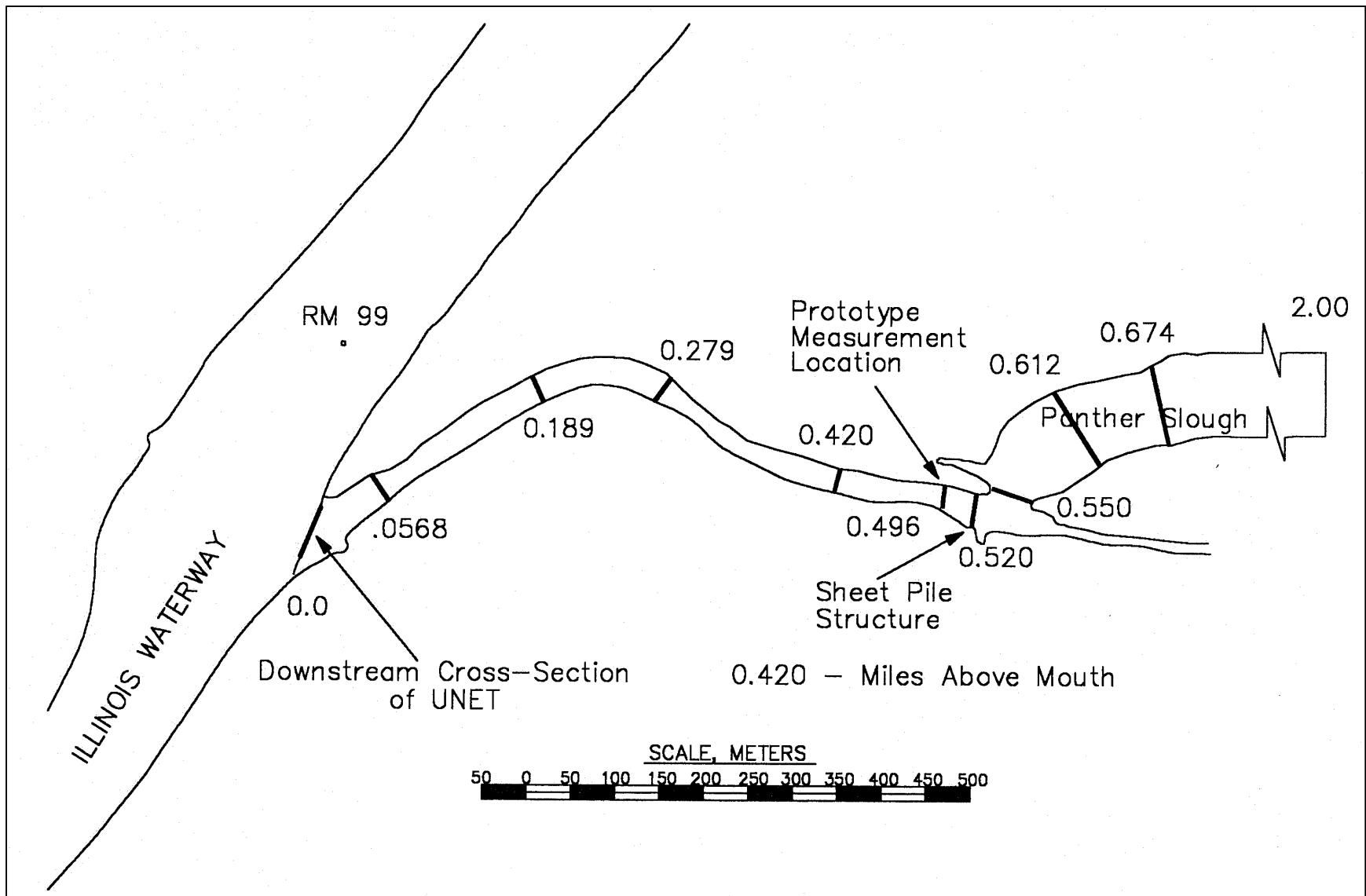
Figure 20. Illinois Waterway Backwater Channel cross-section locations for UNET simulation
