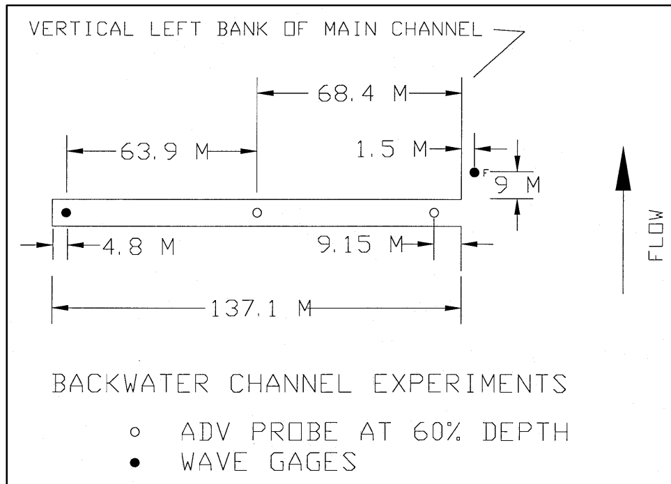
Figure 5. Plan view of physical model backwater and instrument locations
