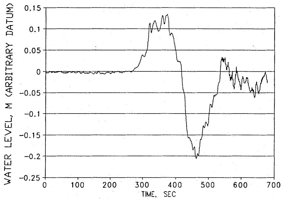
b. Wave gage located inside the backwater channel
