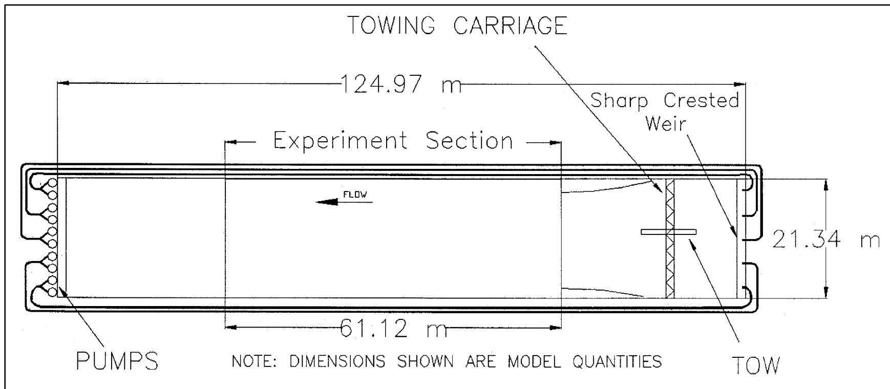
Figure 1. Layout of navigation effects flume
