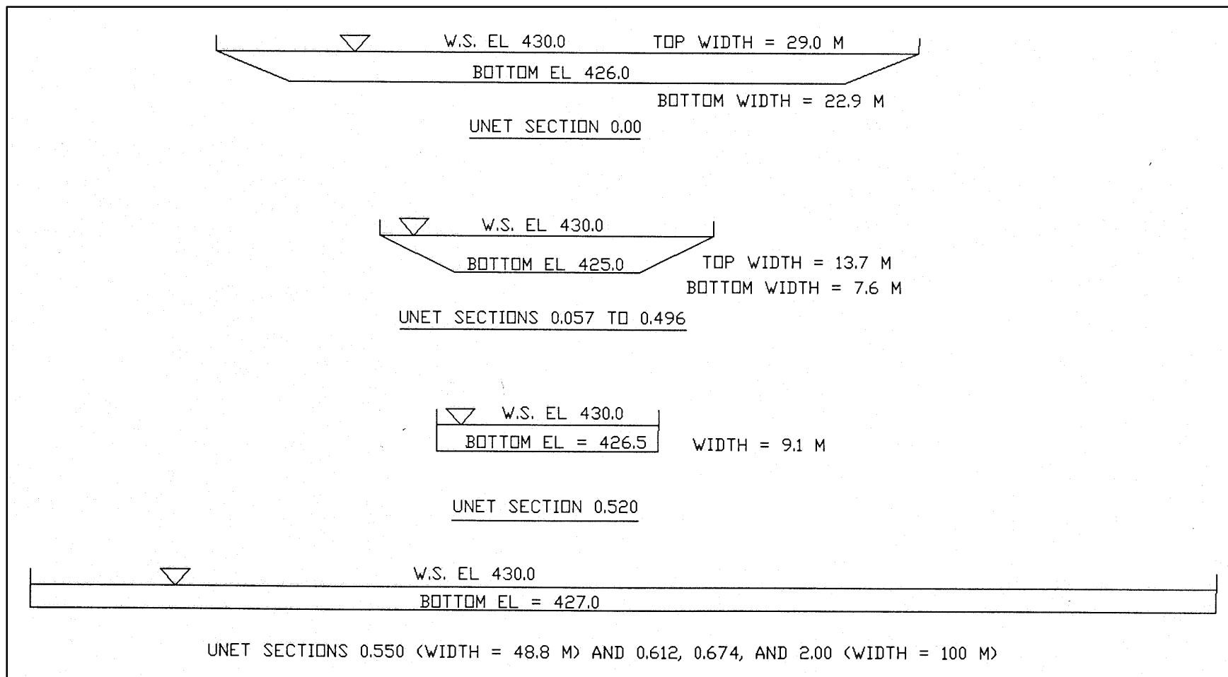
Figure 24. Cross sections used in UNET for Illinois Waterway
