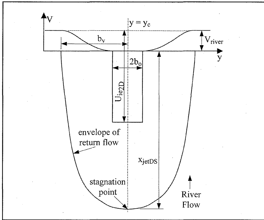
Figure 2. Envelop for counter-flowing jets (no scale)
