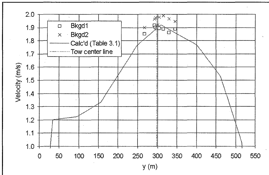
Figure 3. Velocities without towboat and barges
