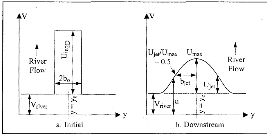
Figure 1. Velocity distributions for co-flowing jets (no scale)
