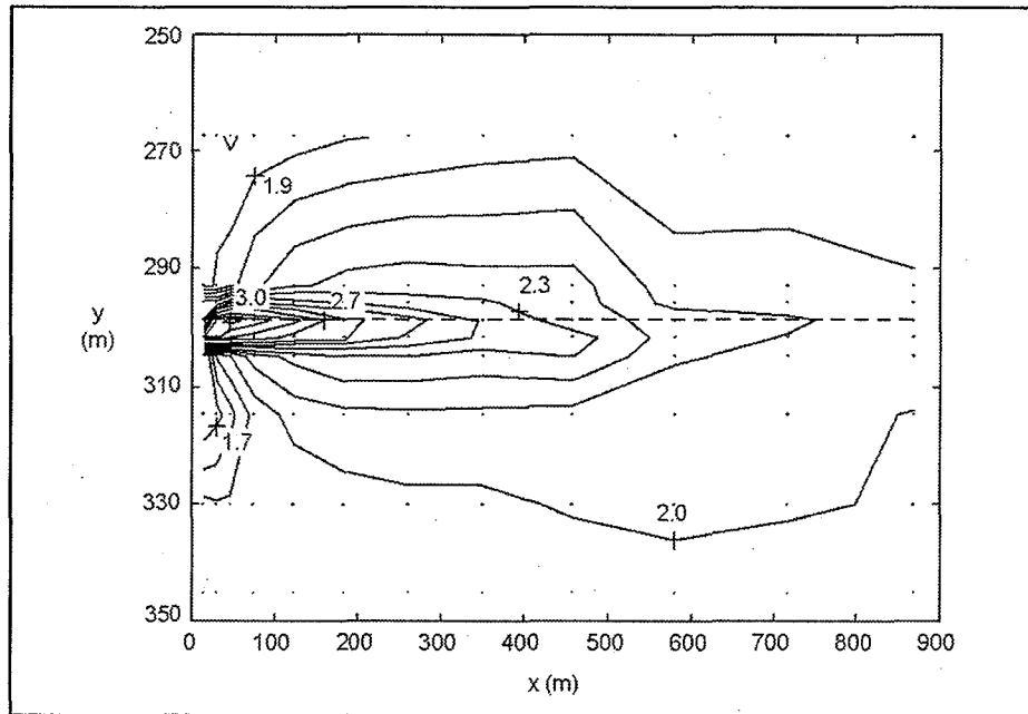
Figure 4. Contours of depth-averaged velocity in m/s
