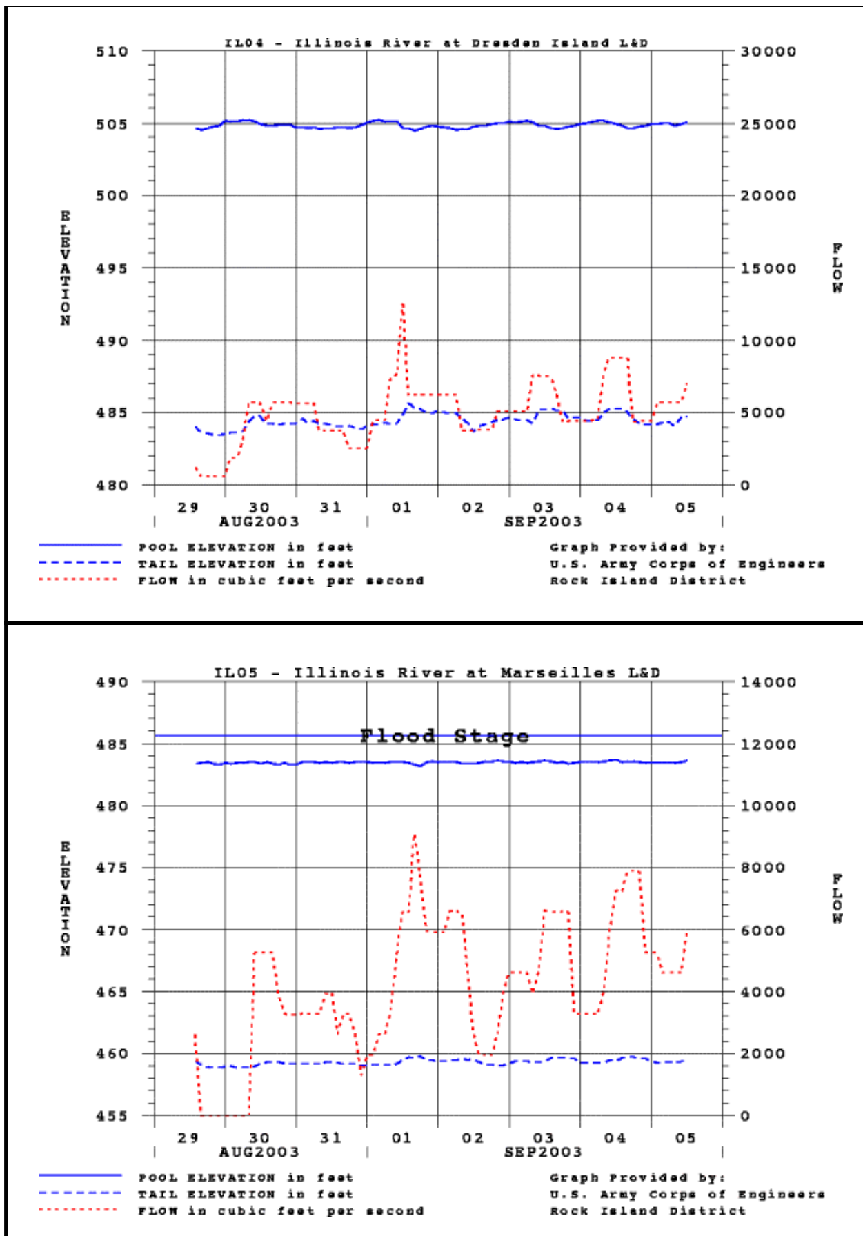
Figure 16. Short-term Water Level Fluctuations on the Illinois Waterway.
