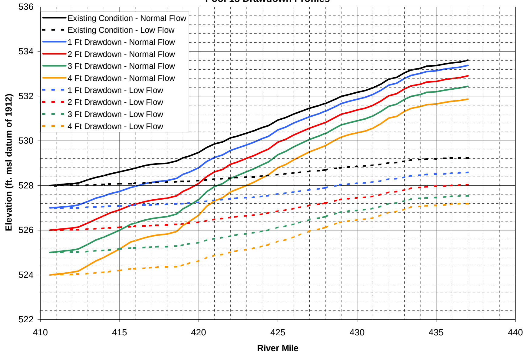
Pool 18 Drawdown Profiles
